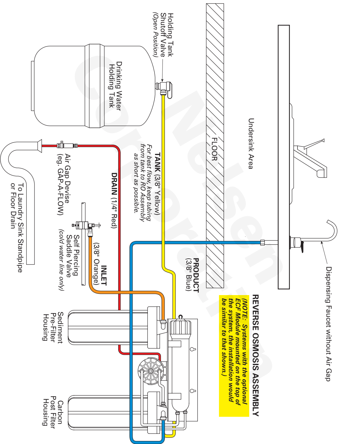
FIGURE 5: General Basement Installation Diagram
